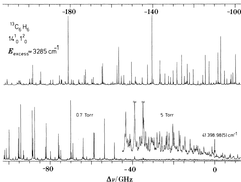
Figure 2. The main traces show part of the {}^{\text{a}}\text{Q} -branch of the 14_0^1 1_0^2 band of ^{13}\text{C}_6\text{H}_6 as excited with the cw laser at a sample pressure of 0.7 Torr†. The typical band-edge seen in regular spectra of benzene cannot be seen, and the observed number of lines is much lower than expected. The insert shows part of the same spectral region at a sample pressure of 5 Torr. Under these conditions the typical rise of the signal strength with decreasing energy away from the band centre as expected for a Q-branch of a totally symmetric two-photon band is observed, and reveals the location of the rotationless origin at \nu_{00} = 41398.98(5) \text{ cm}^{-1} .
