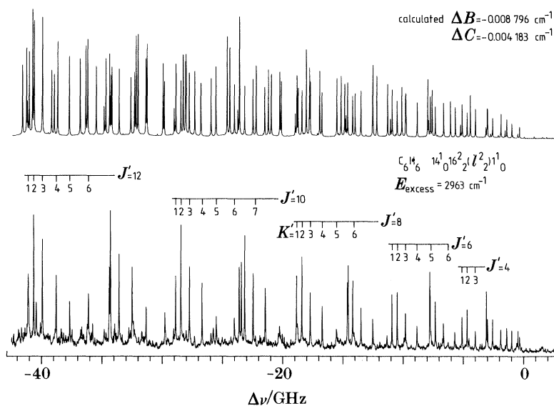
Figure 1. The lower trace shows part of the {}^a\text{Q} -branch of the Doppler-free cw two-photon fluorescence-excitation spectrum of the 14^1_0 1^1_0 16^2_2(l^2_2)1^1_0 band of C_6H_6 at an experimental resolution of 25 MHz. The 14^1_0 1^1_0 16^2_2 state reached by this transition is of particular interest, because its vibrational excess energy of 2963\ \text{cm}^{-1} is very close to the onset of 'channel three' at 3000\ \text{cm}^{-1} . Some assignments are indicated above the spectrum. The upper trace shows the regular {}^a\text{Q} -branch spectrum calculated with the values of the rotational constants determined from the analysis of the experimental spectrum. For a discussion of the differing intensities see text.
